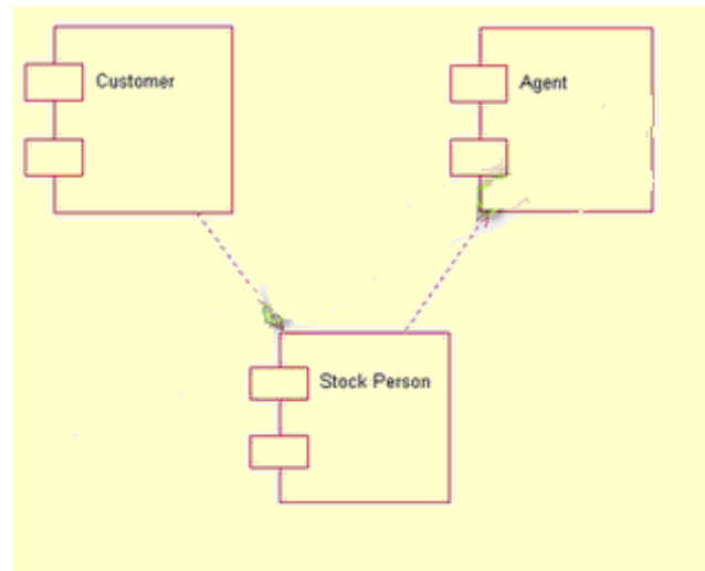
Fig.8.2.COMPONENT DIAGRAM
