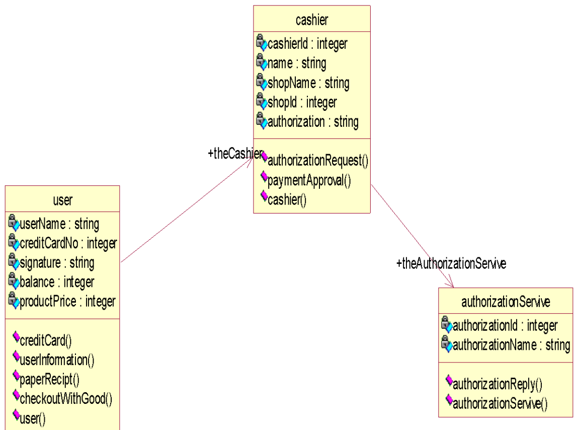
Fig.4.CLASS DIAGRAM
