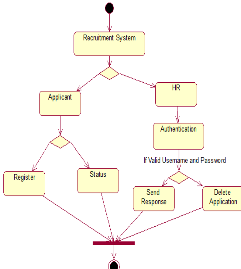
Fig.4. ACTIVITY DIAGRAM
